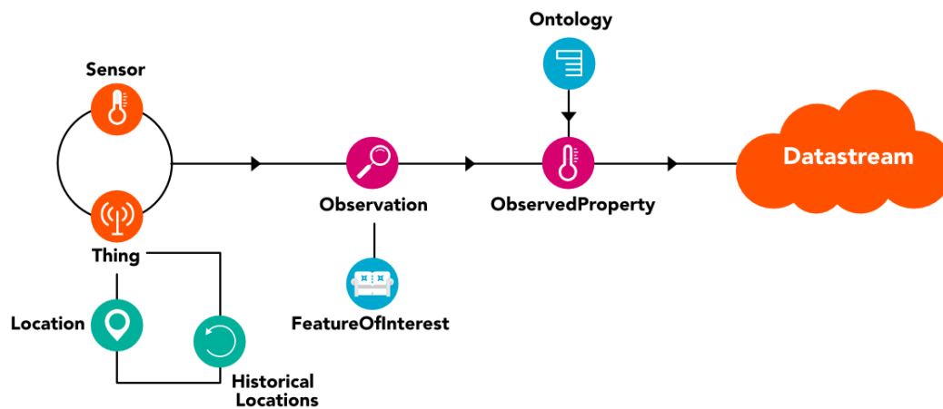
Figure 1: SensorThings API
