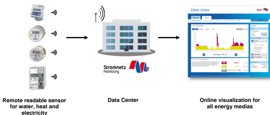
Figure 7-11: system functionality of multi metering system
