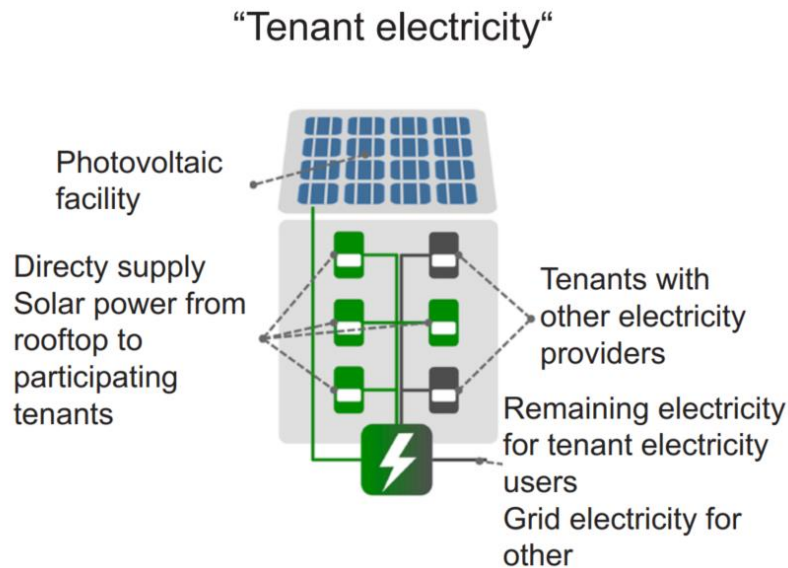
Figure 5-2: Concept of electricity tenant power supply – source: ENH-own
