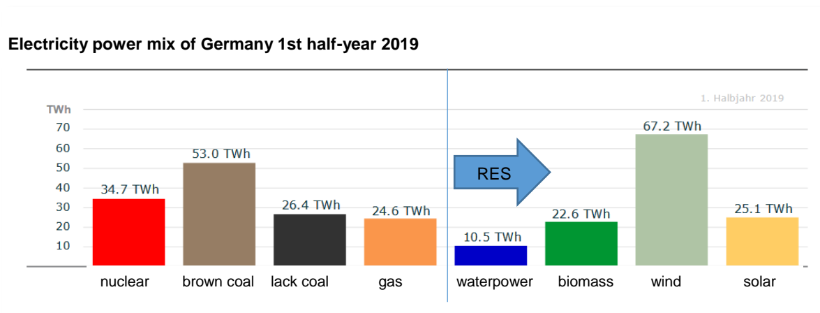
Figure 3-1: Electricity power mix of Germany 1st half-year 2019, Source: Fraunhofer.ise
