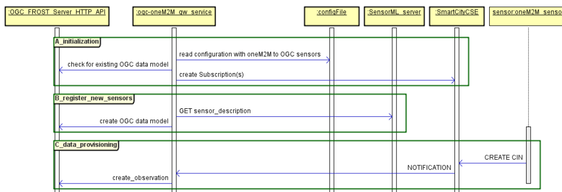
Figure 6: Message flow of the gate service for the oneM2M-to-OGC/STA direction
