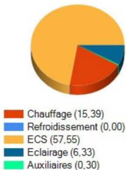
Figure 24: Extract from the French national thermal regulation calculation about the potential consumption in primary energy (kWhPE/m²) after retrofitting; DHW (57.55, in yellow), heating (15.39, in red), lighting (6.33, in blue).
