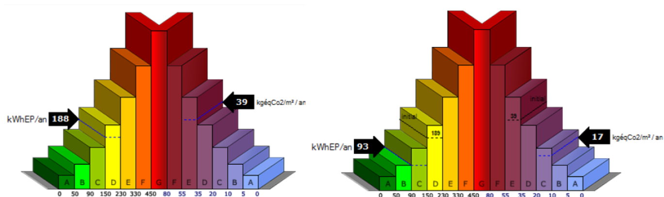
Figure 33: comparison of initial state (left figure) and potential performance after retrofitting (right figure); for primary energy consumption (left side of each figure, in kWhEP/m².year) and CO2 emission (right side of each figure, in kgeqCO2.m².year); Extract from the French national thermal regulation calculation,
